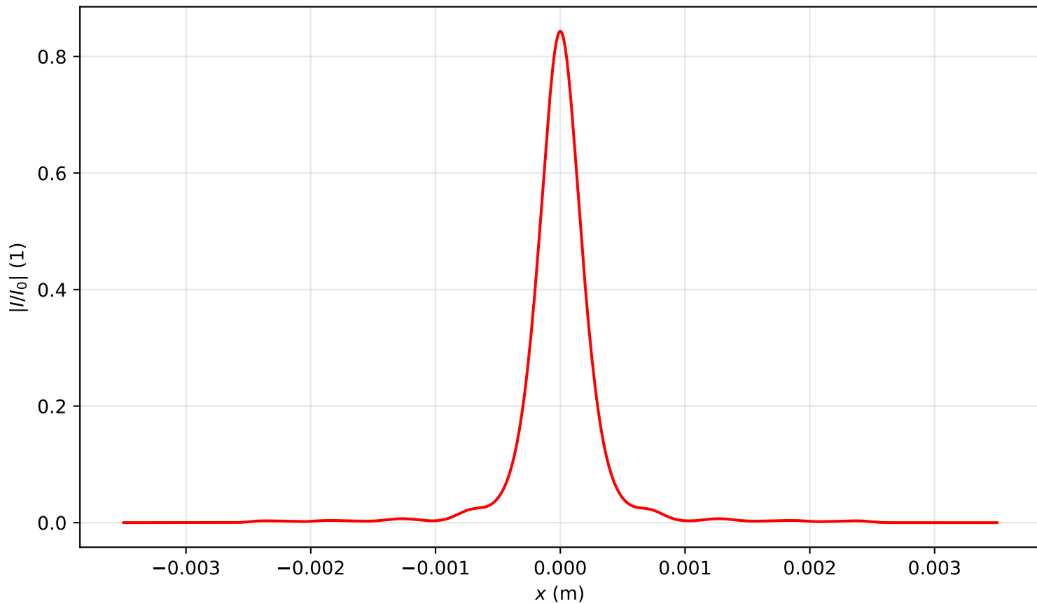
Intensity profile I(x, y = 0, z = 3.662)/I_0 , \text{Pin}=3.0\text{Pcr} , artificial time
